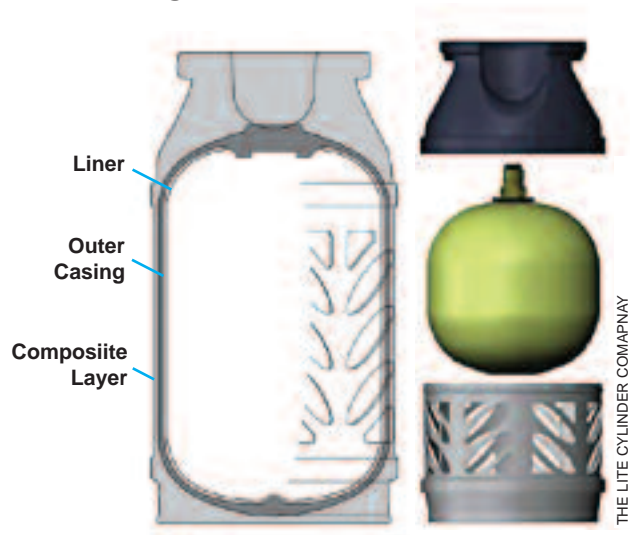
Figure 5 One-piece construction composite cylinders.
